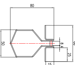
Channel profile M(1:1)
