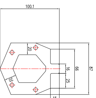
Position 2: flange for H80 M(1:1)
