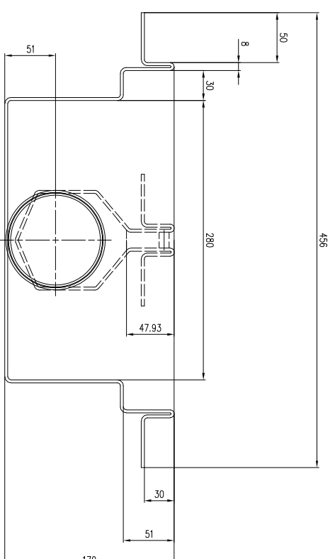
t=1.5mm Rmin=t
