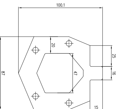
Flange for H80 M(1:1)
