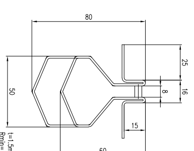
Channel profile M(1:1)
