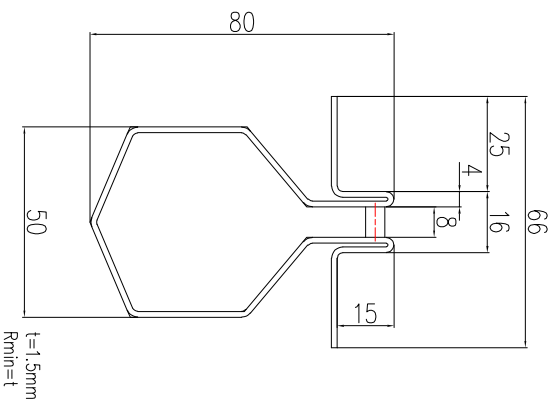
Channel profile M(1:1)
