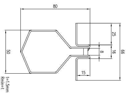
Channel profile M(1:1)
