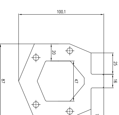
Flange for H80 M(1:1)
