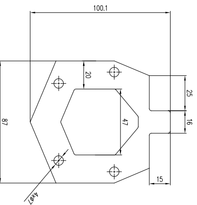
Flange for H80 M(1:1)
