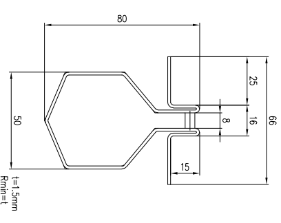
Channel profile M(1:1)
